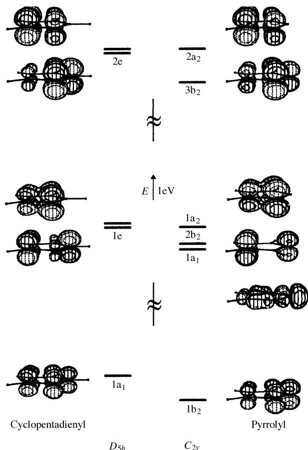
Fig. 7 Cyclopentadienyl vs. pyrrolyl comparative MO diagram
